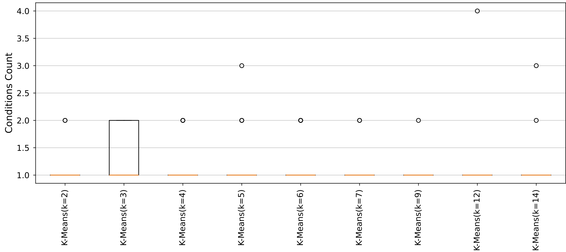
YARA Rules Conditions Count Distribution (Cluster7_Size14 dataset)
